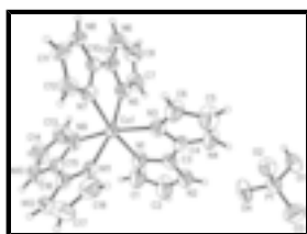
Fig. 1. A view of the structure of complex. Ellipsoids are drawn at the 30% probability level.
